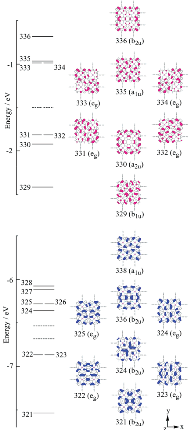
Figure 4. Frontier molecular orbital diagram and contour plots of occupied and virtual orbitals of 3_{\text{Ph}} (TDHF-ZINDO/S). The dotted lines indicate four frontier molecular orbitals of D_{4h} zinc tetraphenylporphyrin (Zn-TPP).
